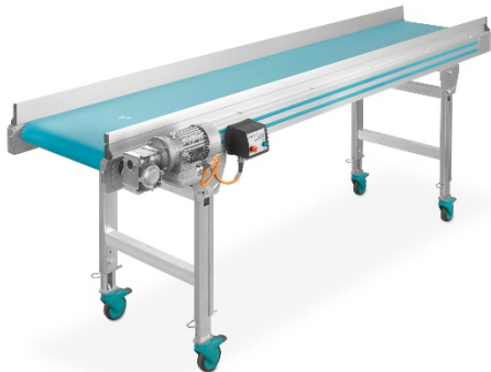
Model: Standard Flat Conveyor (PA 110)
