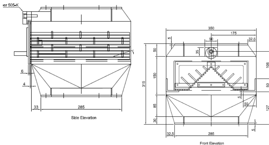
Silo suction box with angel hair drawer built in
